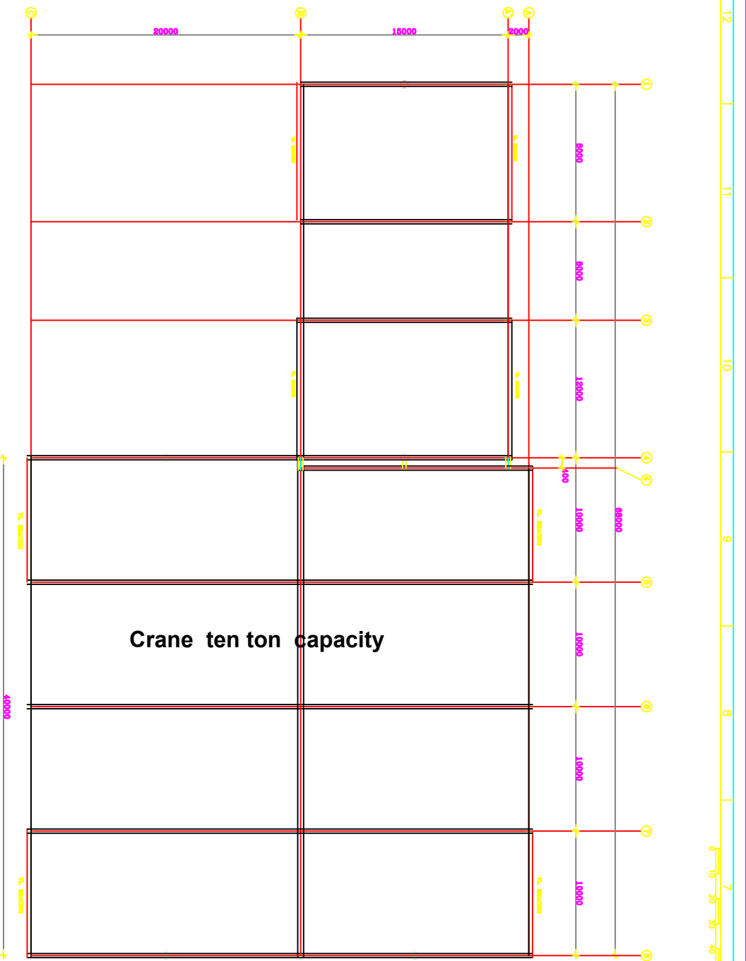
ROOF PLAN
