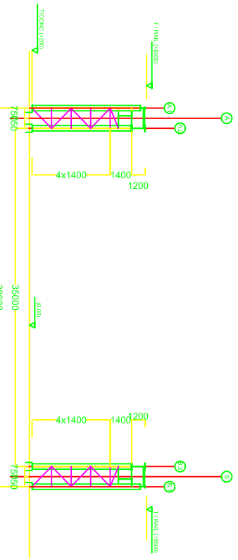
TYPICAL FRAME AT AXES (1, 2, 3)
