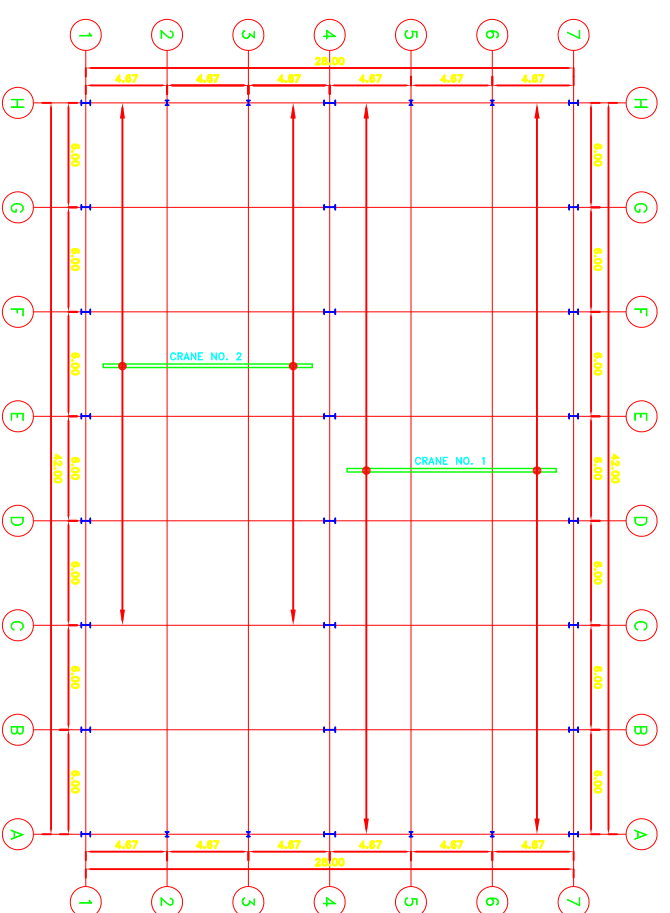
CRANES PLAN
