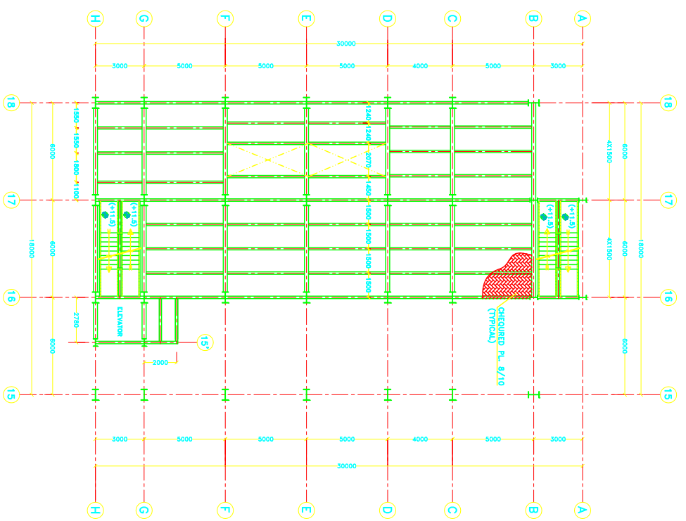
PLAN @ ELEV. (+11.50)
