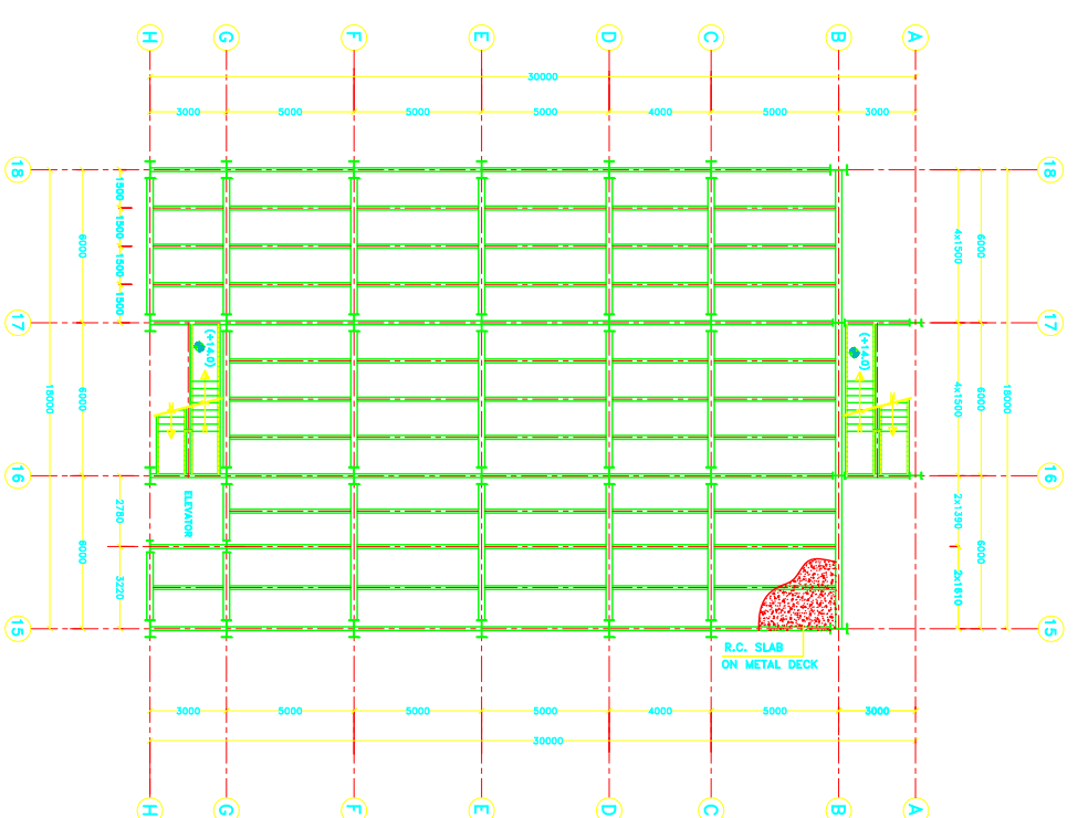
PLAN @ ELEV. (+14.00)
