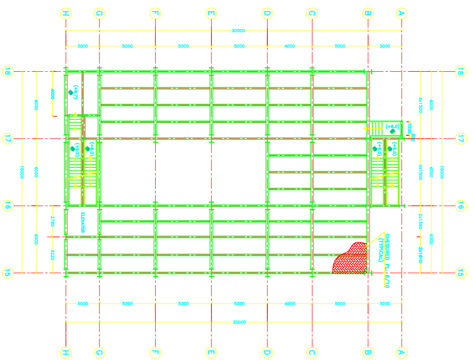
PLAN @ ELEV. (+6.70)
