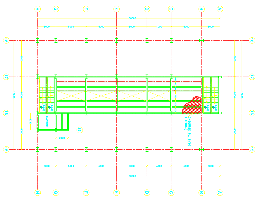
PLAN @ ELEV. (+4.50)
