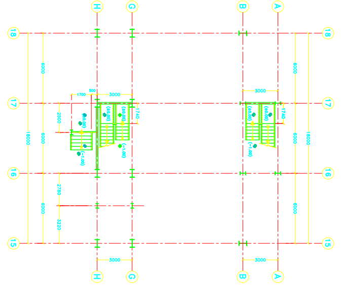
COLUMNS' ARRANGEMENT PLAN @ ELEV. (+1.00)
