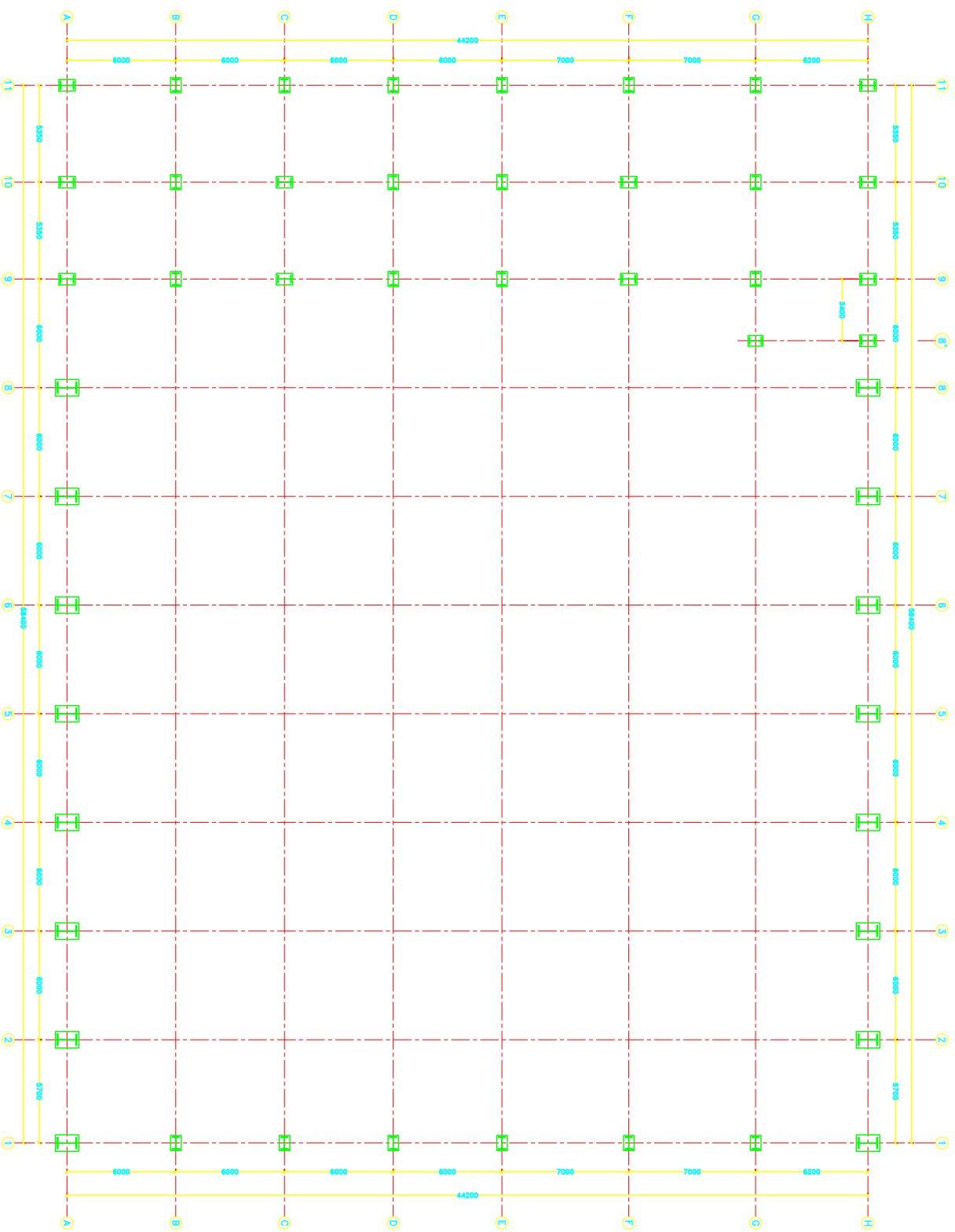
COLUMNS' ARRANGEMENT AT LEVEL (+0.00)
