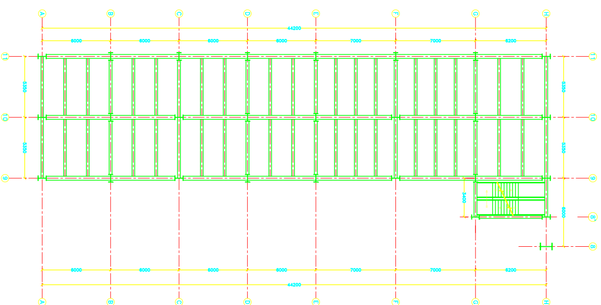
MEZZANINE PLAN (I/STEEL +5.90)
