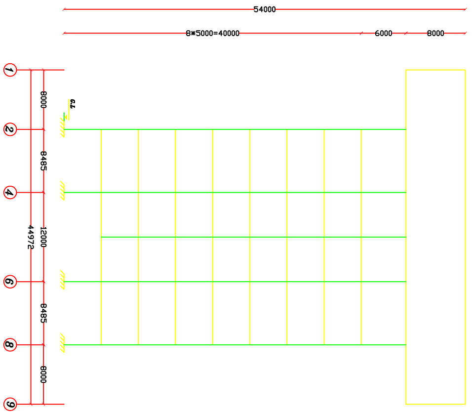
SECTION ELEVATION
